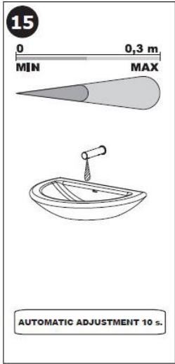
Once power turned on, faucet will automatically adjust sensing range during first 10 seconds. The LED on sensor will continually flash, do not come in active range during this time
